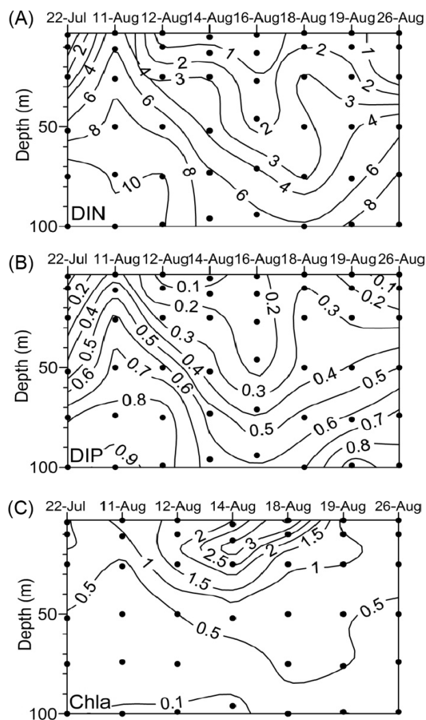
Fig. 4. Vertical profiles of the concentrations of (A) dissolved organic nitrogen (DIN, \text{NO}_3 + \text{NO}_2 ), (B) dissolved inorganic phosphate (DIP), and (C) chlorophyll a (chl a). No profile of chl a concentration was obtained on 16 August
