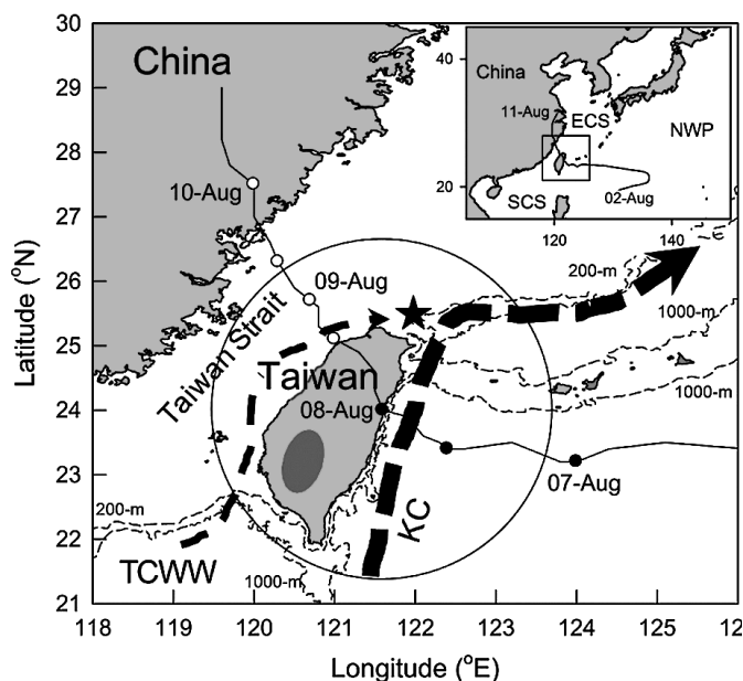
Fig. 1. Track of Typhoon Morakot and the location of the observation station in the southern East China Sea. The complete route of Morakot from 2 to 11 August is shown in the upper right panel. NWP, ECS, and SCS denote the North-western Pacific, the East China Sea, and the South China Sea, respectively. The small solid and open circles denote the strength of Morakot at levels of category-2 (maximum wind speed = 43 \text{ m s}^{-1} ) and category-1 (maximum wind speed = 33 \text{ m s}^{-1} ), respectively. The large circle represents the area where the wind speed was above 14 \text{ m s}^{-1} . The arrows indicate the flow directions of the Kuroshio Current (KC) and the Taiwan Current Warm Water (TCWW; Gong et al. 1996, Jan et al. 2010, 2011). The location of the observation station is indicated by a star. The Morakot-induced flooding region in southern Taiwan is shaded dark gray
