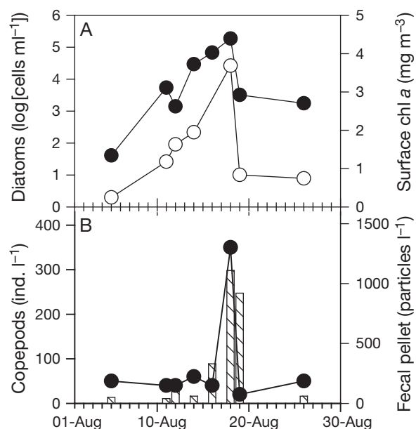
Fig. 6. (A) Surface total diatom abundance (●) and chlorophyll a (chl a ) concentration (○). (B) Surface copepod abundances (●) and their fecal pellet concentrations (bars) at a depth of 50 m
