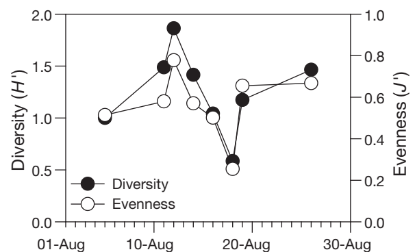
Fig. 5. Indices of biological diversity ( H' ) and evenness ( J' ) for the assemblages of microphytoplankton pre- and post-Typhoon Morakot
