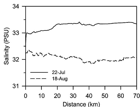
Fig. 3. Surface salinity along the ship track from the north coast of Taiwan at Keelung Harbor (25.17° N, 121.80° E) to the study site. The salinities pre- and post-Typhoon Morakot are denoted by the solid and dashed lines, respectively
